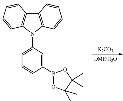
Compound (IV)
