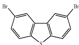
Compound (I)
