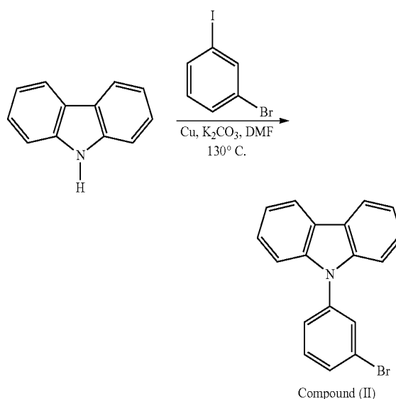
Compound (II)
